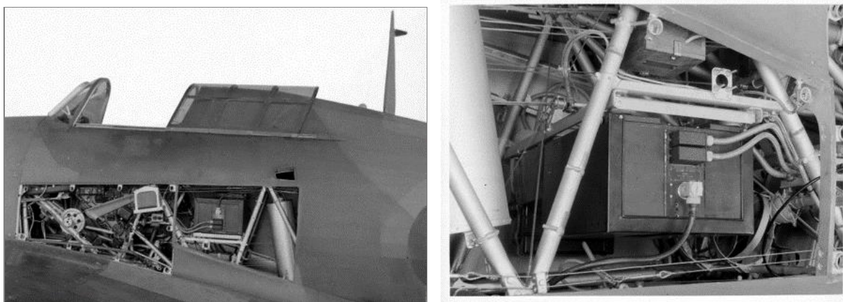
Figure 30. The fitting to the experimental TR1133 VHF radio system to the RAE Hurricane (L1788) photographed on the 18th September 1939
